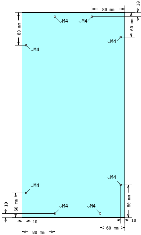
DRAWING 5, Pos 10 Hole placement
