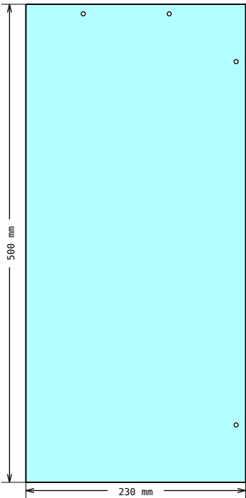
DRAWING 3, Pos 8 Shape measurements
