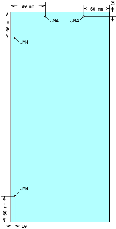
DRAWING 1, Pos 6 Hole placement
