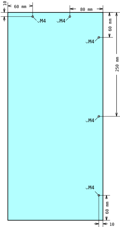
DRAWING 2, Pos 7 Hole placement
