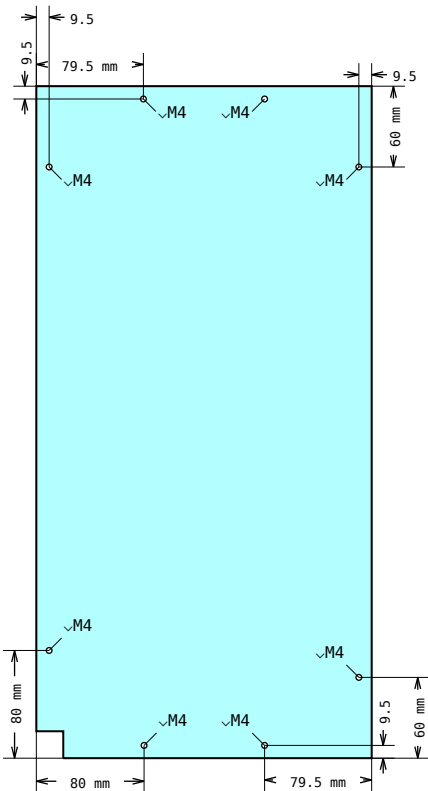
DRAWING 4, Pos 9 Hole placement
