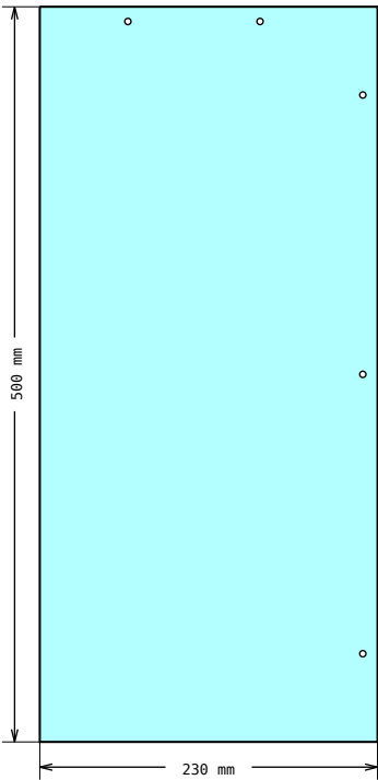
DRAWING 2, Pos 7 Shape measurements
