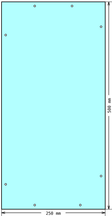
DRAWING 5, Pos 10 Shape measurements
