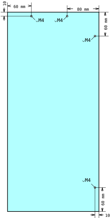
DRAWING 3, Pos 8 Hole placement
