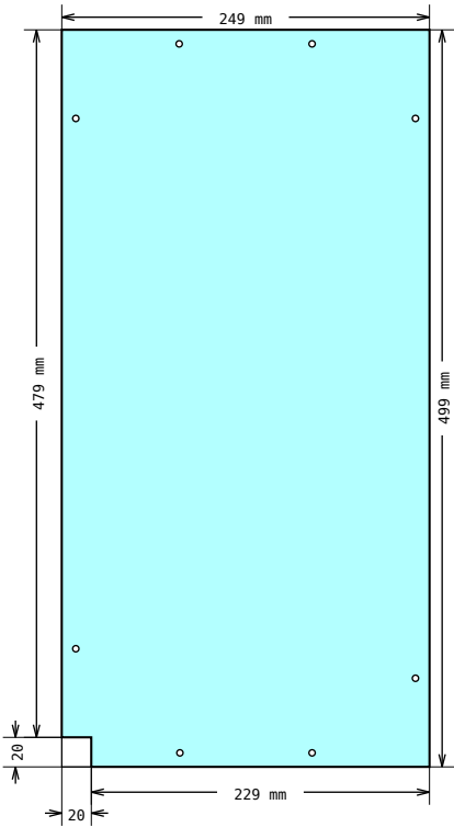
DRAWING 4, Pos 9 Shape measurements
